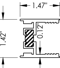
5 FIXED STILE
