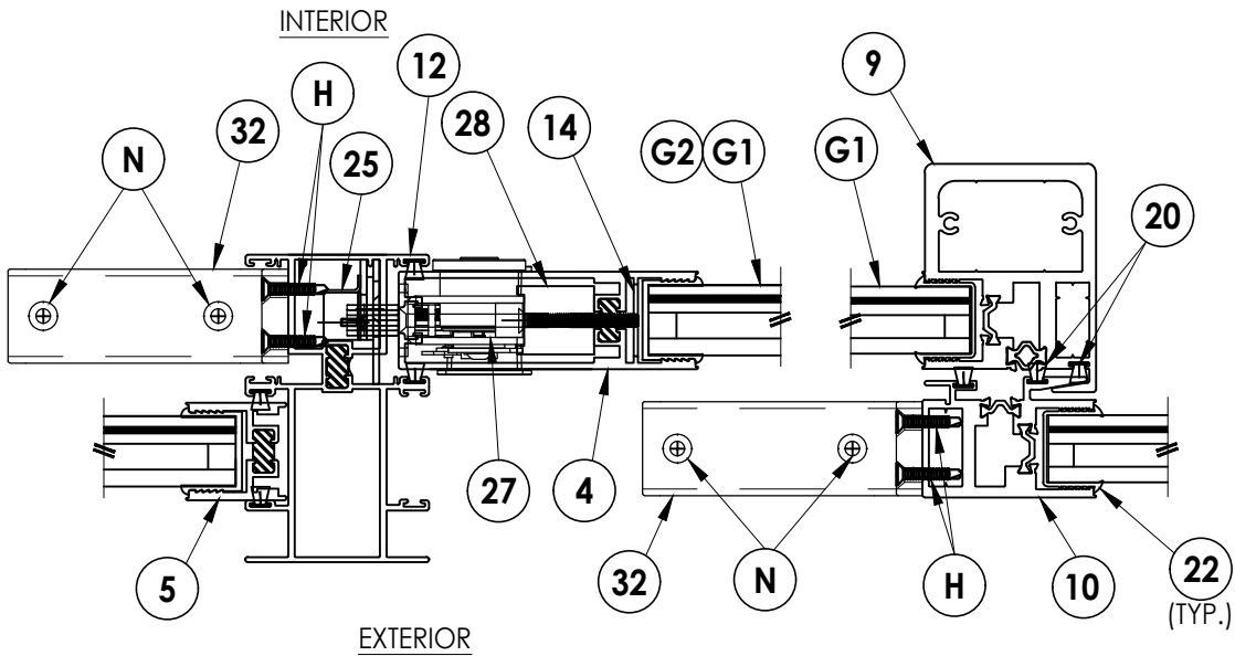
1 2 HORIZONTAL CROSS SECTION 2X Buck Construction
