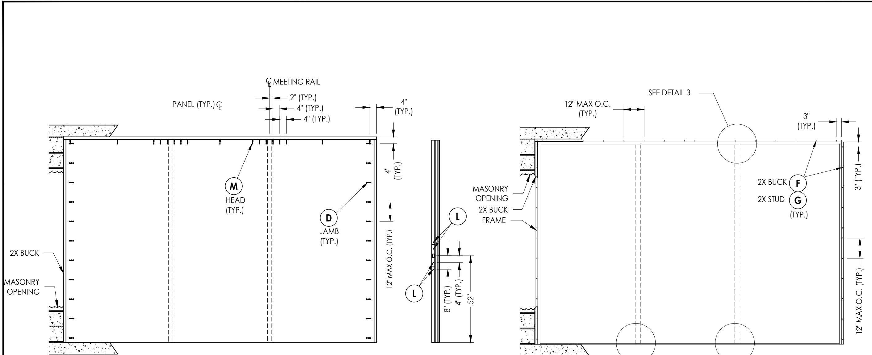
2X BUCK ANCHORING Sliding Glass Door
