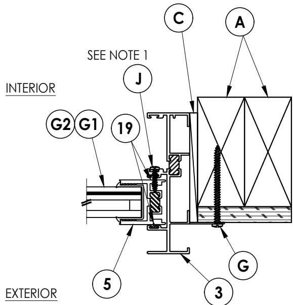
2 2 HORIZONTAL CROSS SECTION 2X Stud Construction
