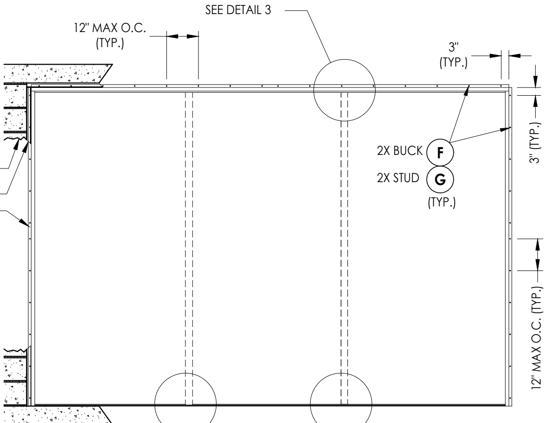
FRAME ANCHORING Sliding Glass Door
