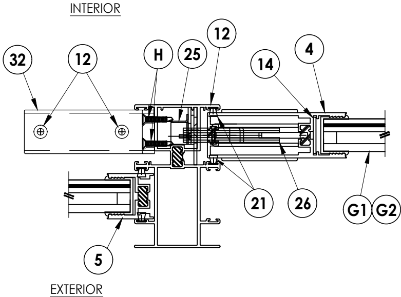
3 2 HORIZONTAL CROSS SECTION
